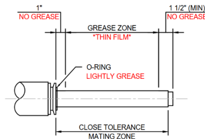
Picture 10 – Close Tolerance V-Band Style Male
