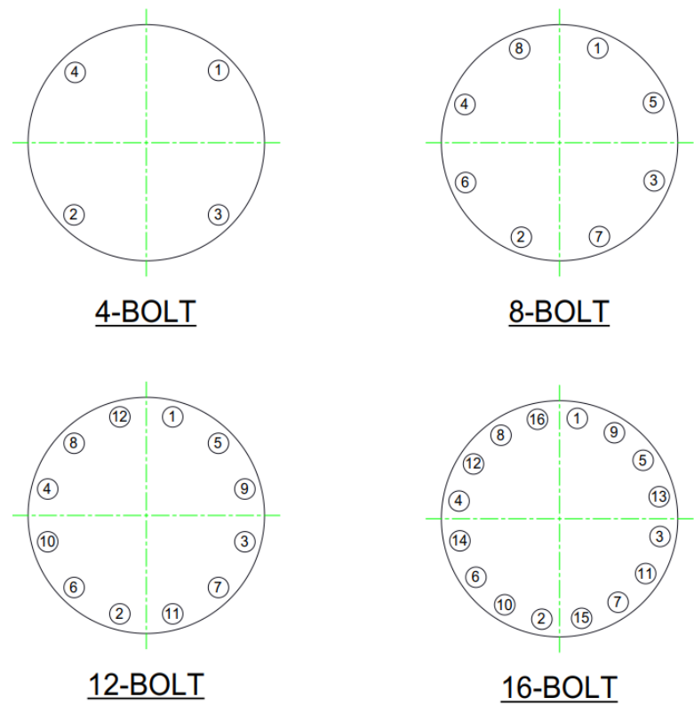
Picture 19 – Torque Sequence
