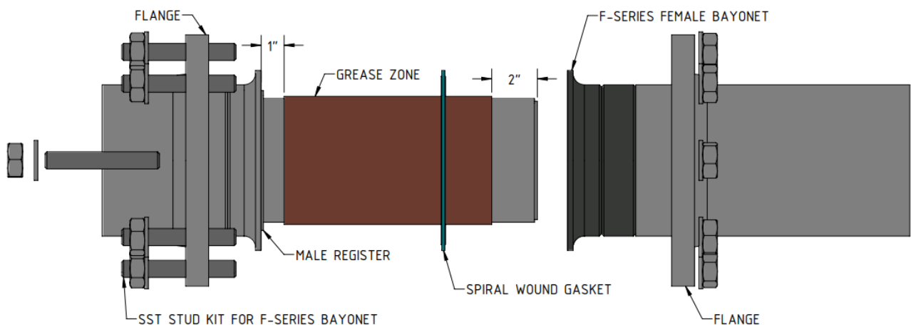
Picture 16 – F- Series Bayonet
