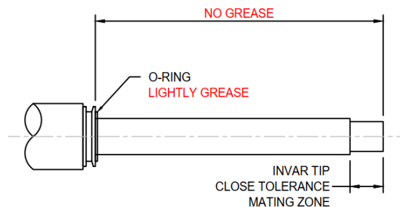
Picture 11 – Invar Tip Style Male Bayonet
