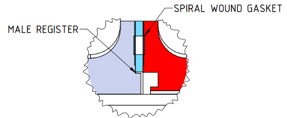
Picture 18 – Gasket Fit Up
